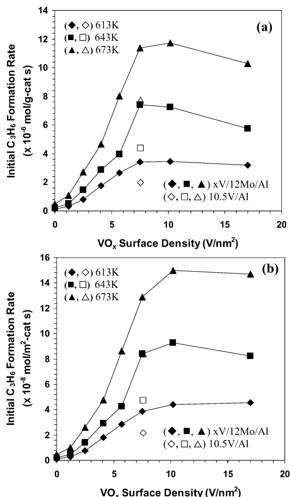
Fig. 4. Effects of VO_x surface density on the initial rates of C_3H_6 formation per gram of catalyst (a) and per unit surface area of catalyst (b).
