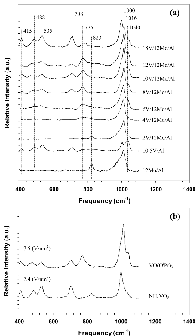
Fig. 1. (a) Raman spectra of 12Mo/Al, 10.5V/Al, and xV/12Mo/Al ( x = 2 –18). (b) Raman spectra of a monolayer of vanadia dispersed on 12Mo/Al, prepared from VO(O^iPr)_3 and NH_4VO_3 .
