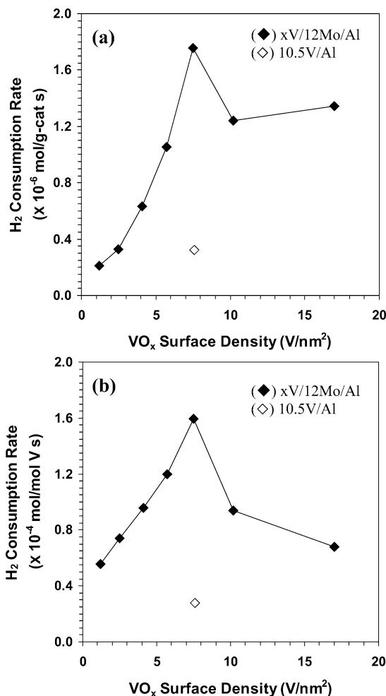
Fig. 6. Effects of VO_x surface density on the rates of H_2 consumption during TPR expressed per gram of catalyst (a) and per mole of V (b) for xV/12Mo/Al ( x = 2-18 ) and 10.5V/Al .
