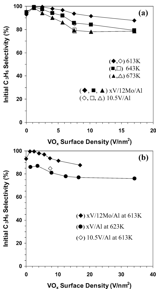
Fig. 7. (a) Effects of VO x surface density on the initial C 3 H 6 selectivities for xV/12Mo/Al ( x = 2 –18) and 10.5V/Al. (b) Comparison of the effects of VO x surface density on the initial C 3 H 6 selectivities for xV/12Mo/Al ( x = 2 –18), xV/Al ( x = 2 –30), and 10.5V/Al.
